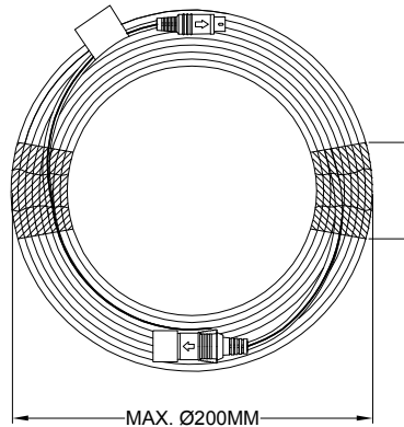
CABLE BINDING SPEC.
